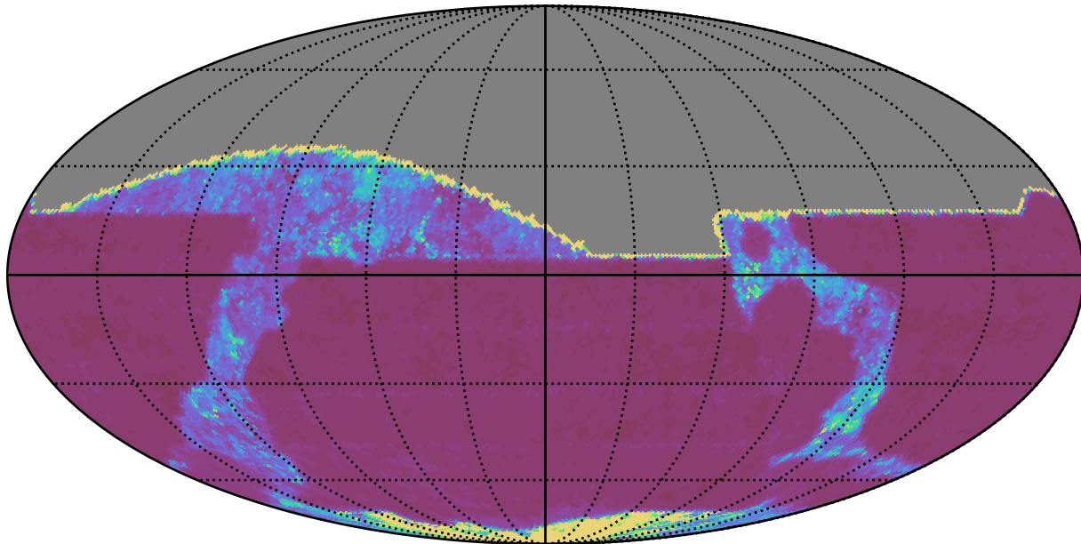
ddf_half_v3.4_10yrs All sky r band: 20thPercentile Inter-Night Gap
