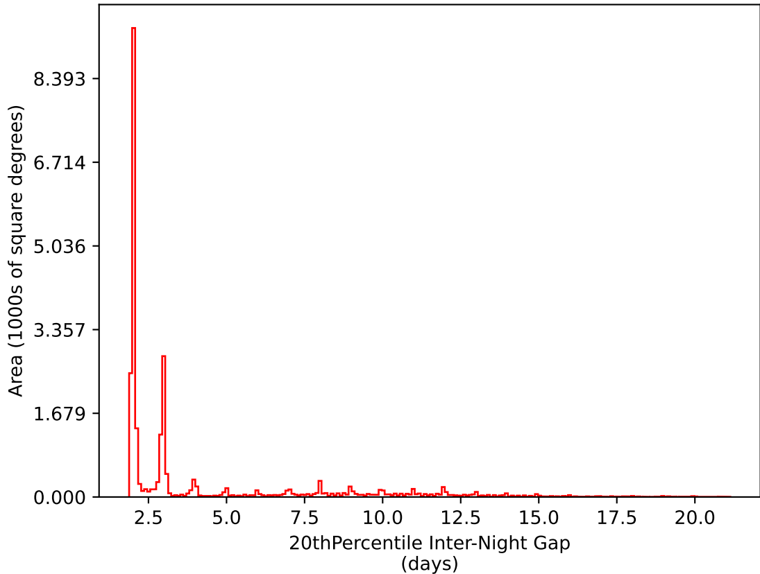
ddf_half_v3.4_10yrs All sky i band: 20thPercentile Inter-Night Gap
