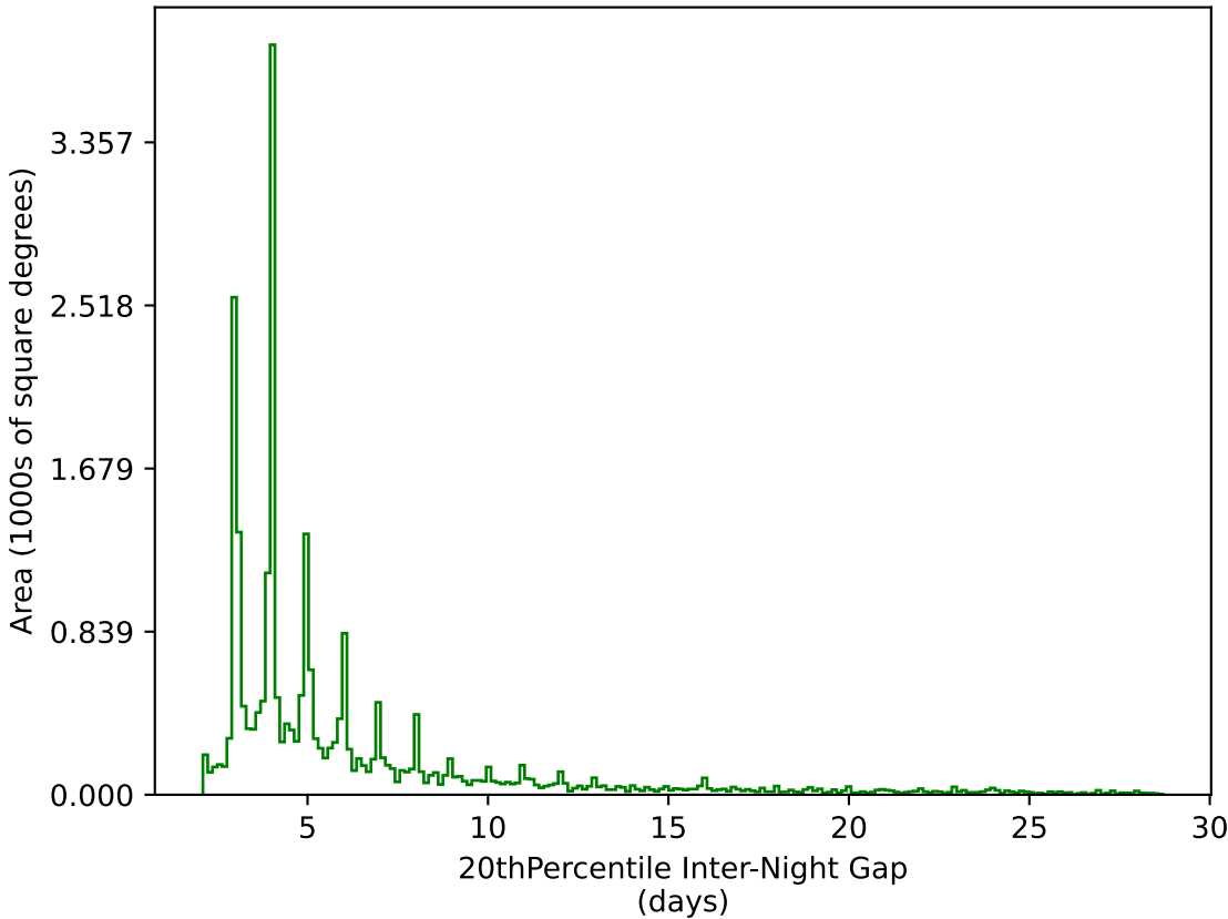
ddf_half_v3.4_10yrs All sky g band: 20thPercentile Inter-Night Gap
