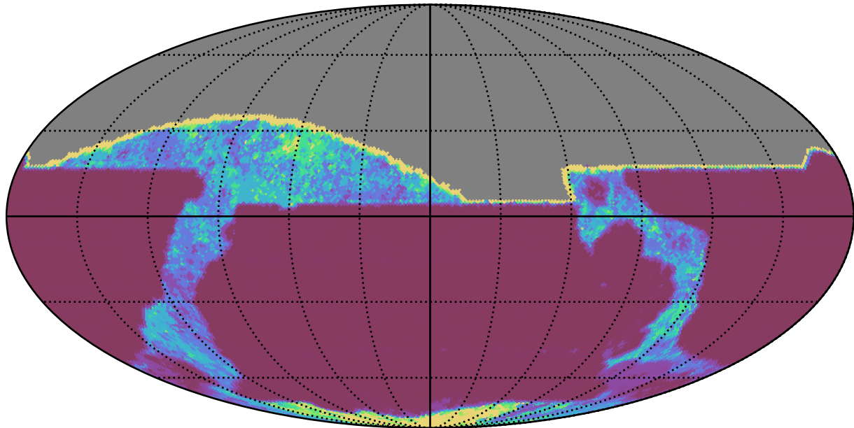
ddf_half_v3.4_10yrs All sky all bands: 20thPercentile Inter-Night Gap
