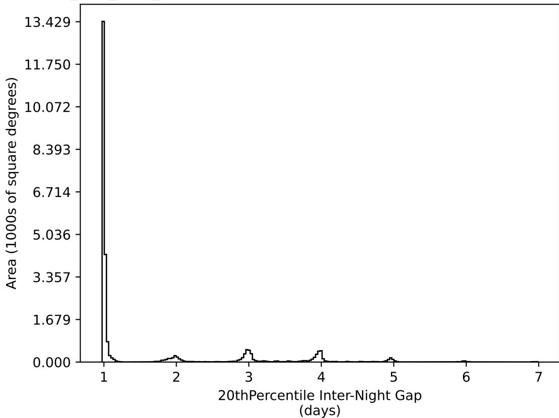
ddf_half_v3.4_10yrs All sky all bands: 20thPercentile Inter-Night Gap
