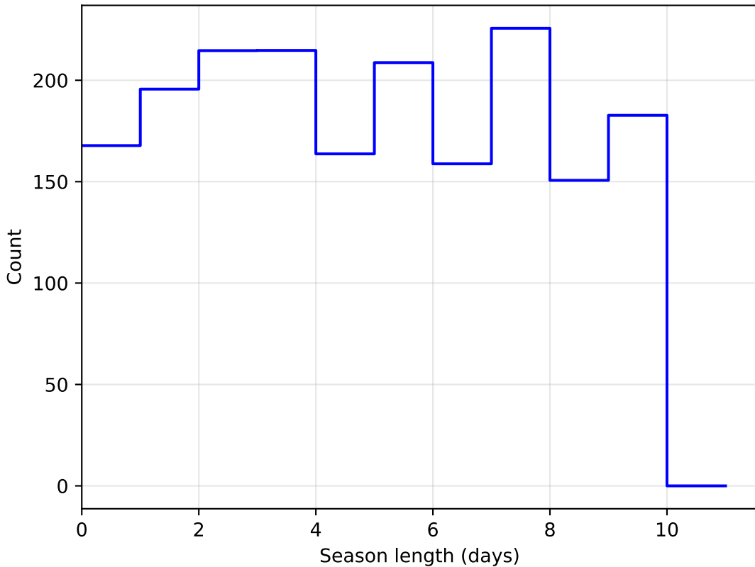
ddf_half_v3.4_10yrs DD:WFD all bands: SeasonLength
