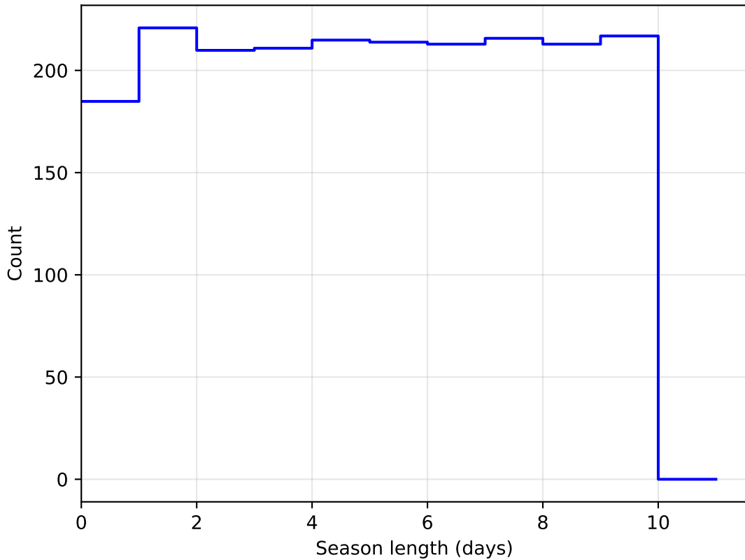
ddf_half_v3.4_10yrs DD:ELAISS1 all bands: SeasonLength
