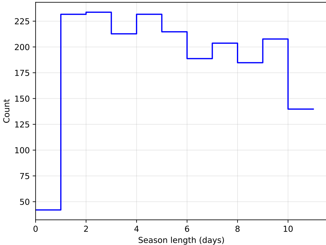
ddf_half_v3.4_10yrs DD: COSMOS all bands: SeasonLength
