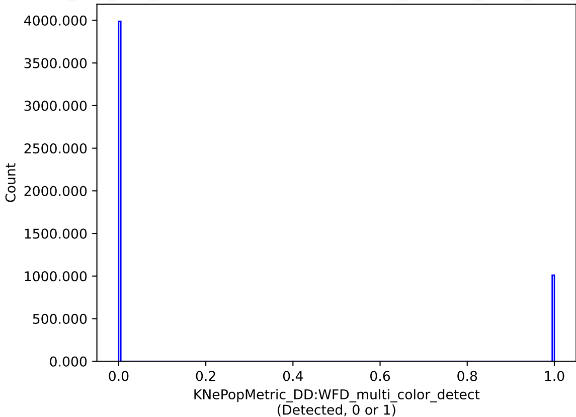
ddf_half_v3.4_10yrs DD:WFD: KNePopMetric_DD:WFD_multi_color_detect
