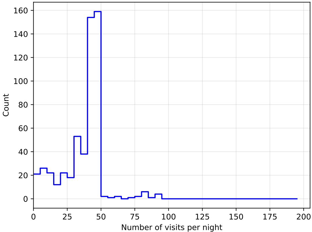
ddf_half_v3.4_10yrs all bands: DD:XMM_LSS NVisitsPerNight
