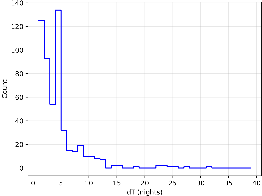
ddf_half_v3.4_10yrs all bands: DD:XMM_LSS Delta Nights Histogram
