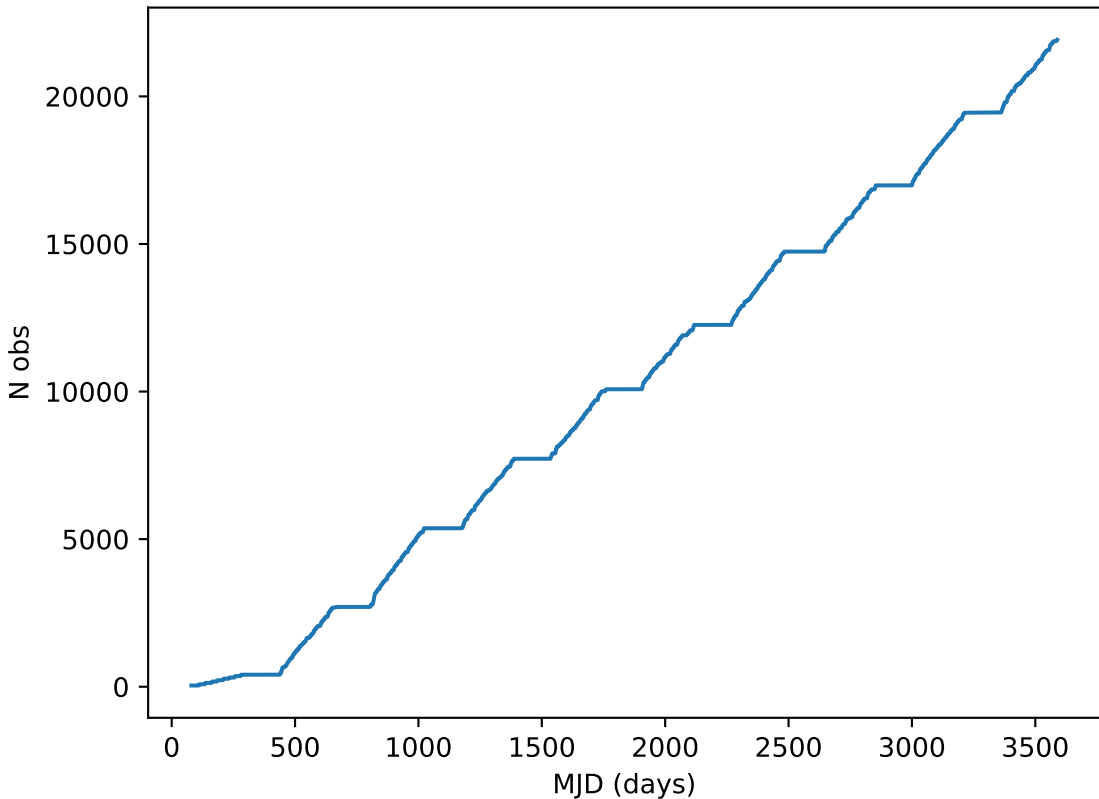
ddf_half_v3.4_10yrs all bands: DD:XMM_LSS Cumulative NVisits
