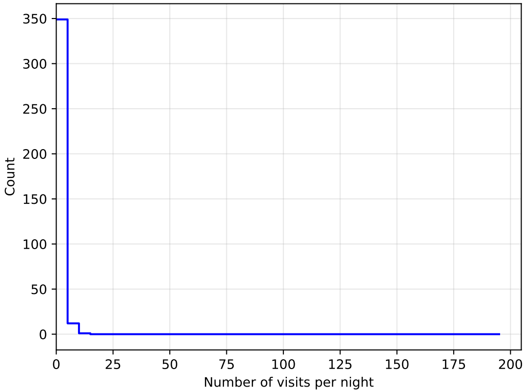
ddf_half_v3.4_10yrs all bands: DD:WFD NVisitsPerNight
