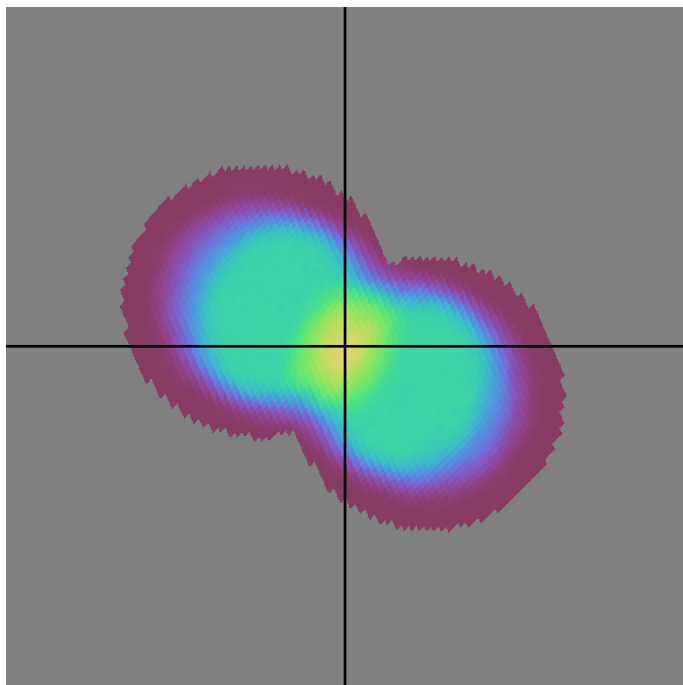
ddf_half_v3.4_10yrs all bands: DD:EDFS NVisits
