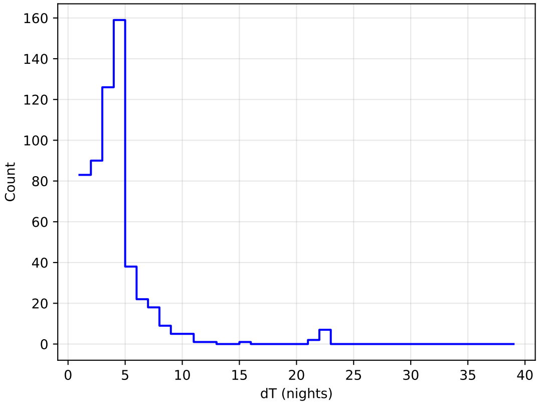
ddf_half_v3.4_10yrs all bands: DD:EDFS Delta Nights Histogram
