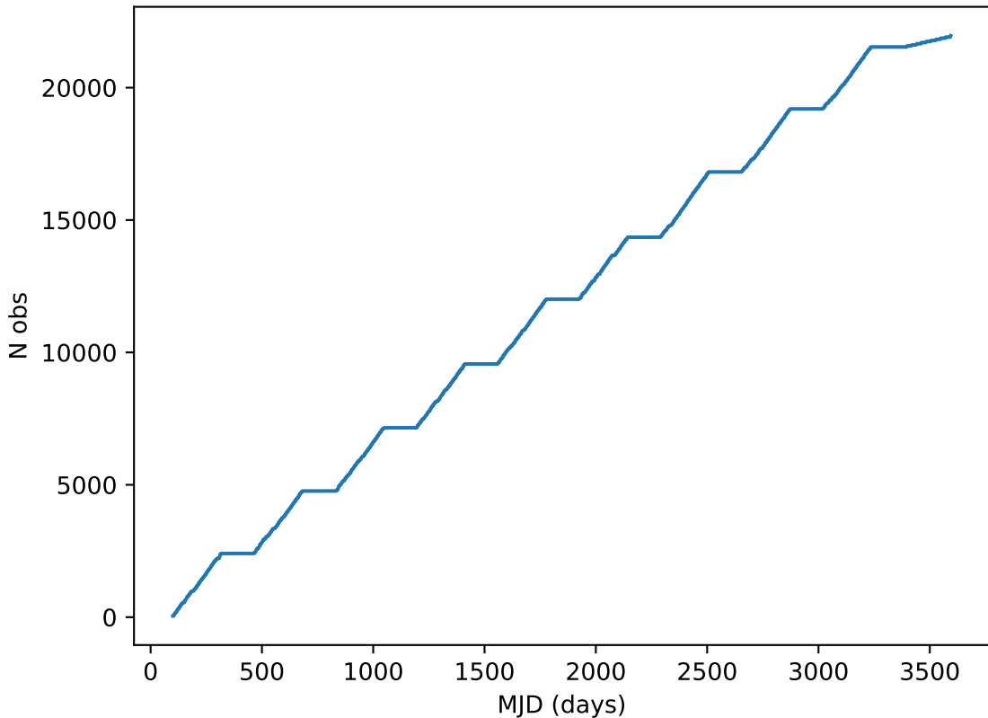
ddf_half_v3.4_10yrs all bands: DD:EDFS Cumulative NVisits
