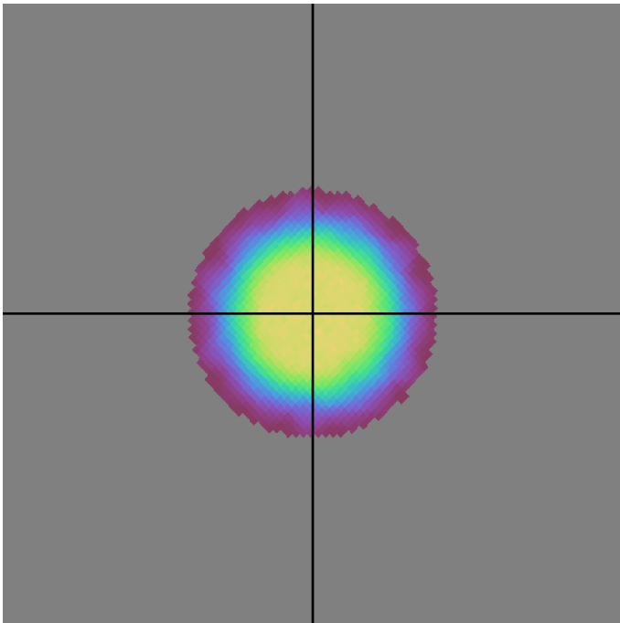
ddf_half_v3.4_10yrs all bands: DD:ECDFS NVisits
