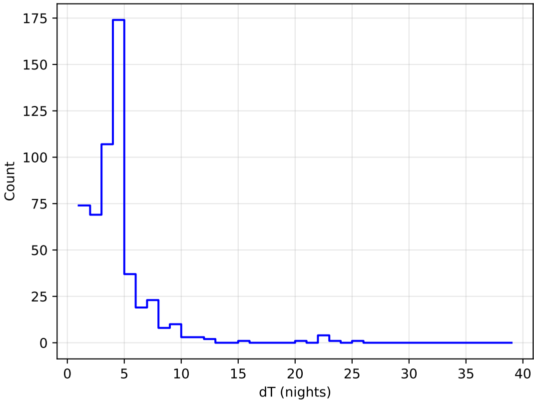
ddf_half_v3.4_10yrs all bands: DD:ECDFS Delta Nights Histogram
