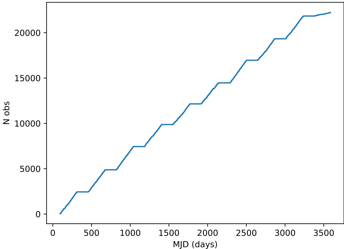
ddf_half_v3.4_10yrs all bands: DD:ECDFS Cumulative NVisits
