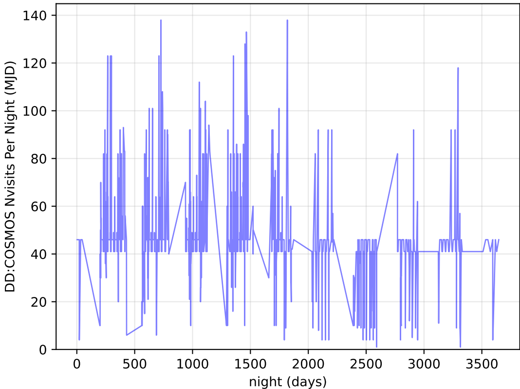
ddf_half_v3.4_10yrs all bands: DD:COSMOS Nvisits Per Night
