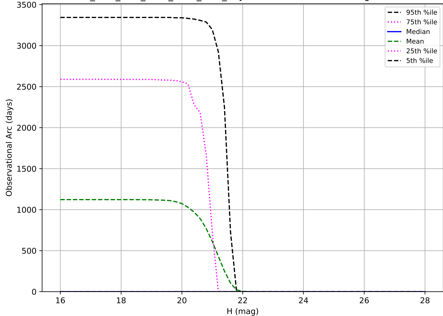
ddf_acor_sf30_lsf40_lsr50_v3.4_10yrs: Observational Arc Length Vatira
