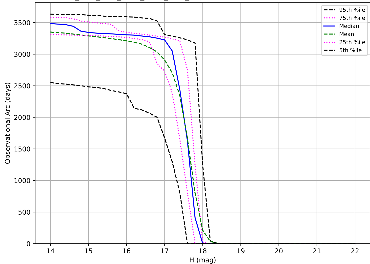
ddf_acor_sf30_lsf40_lsr50_v3.4_10yrs: Observational Arc Length Trojan
