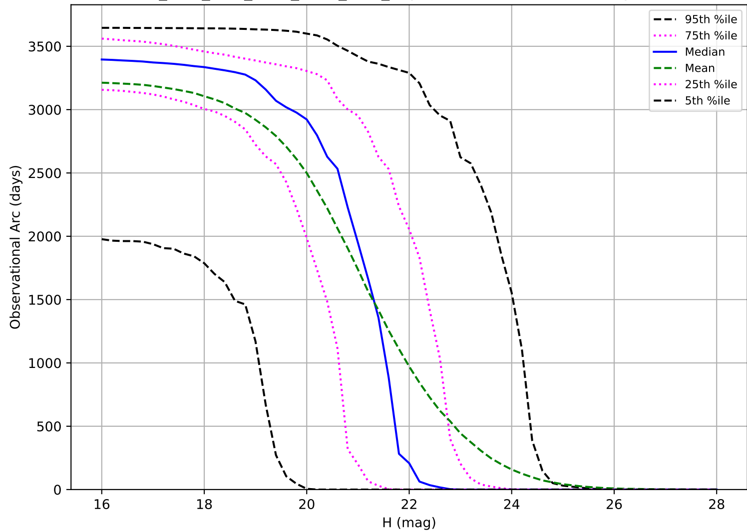
ddf_acor_sf30_lsf40_lsr50_v3.4_10yrs: Observational Arc Length PHA
