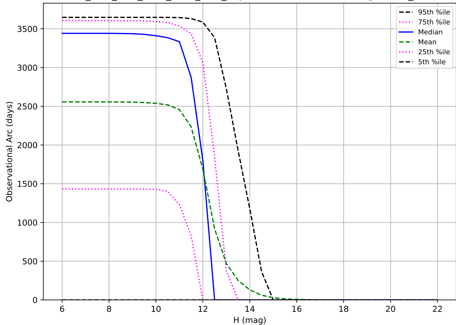
ddf_acor_sf30_lsf40_lsr50_v3.4_10yrs: Observational Arc Length OCC_r20
