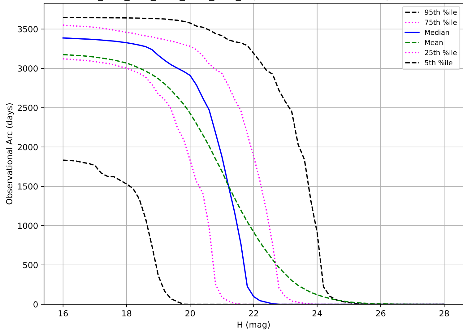
ddf_acor_sf30_Isf40_Isr50_v3.4_10yrs: Observational Arc Length NEO
