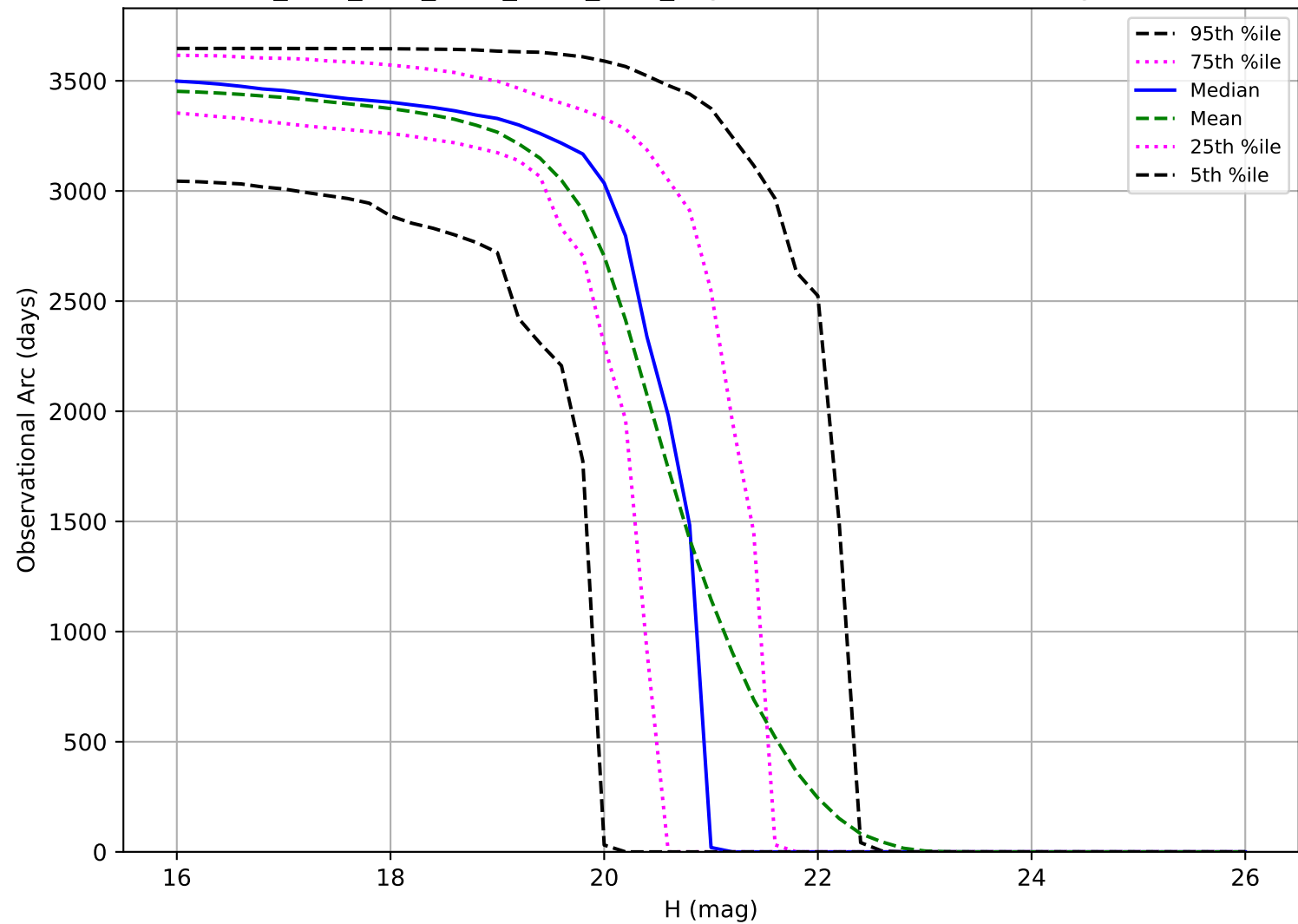
ddf_acor_sf30_lsf40_lsr50_v3.4_10yrs: Observational Arc Length MBA
