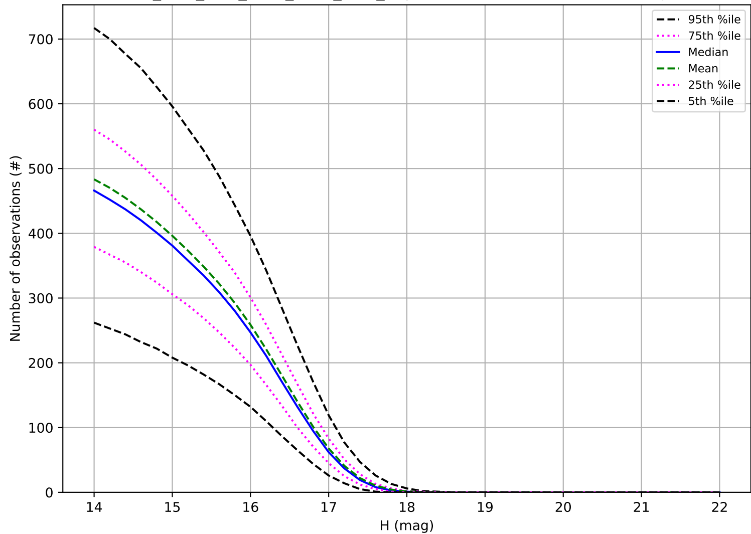
ddf_acor_sf30_lsf40_lsr50_v3.4_10yrs: Number of observations Trojan
