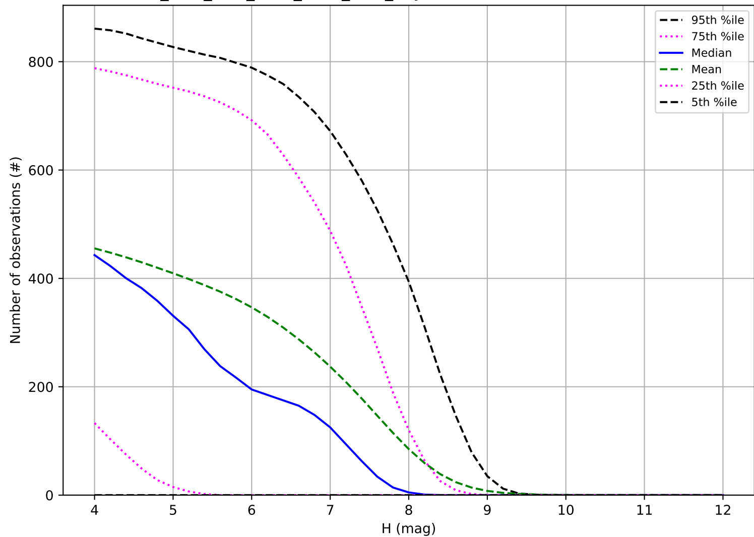
ddf_acor_sf30_lsf40_lsr50_v3.4_10yrs: Number of observations TNO
