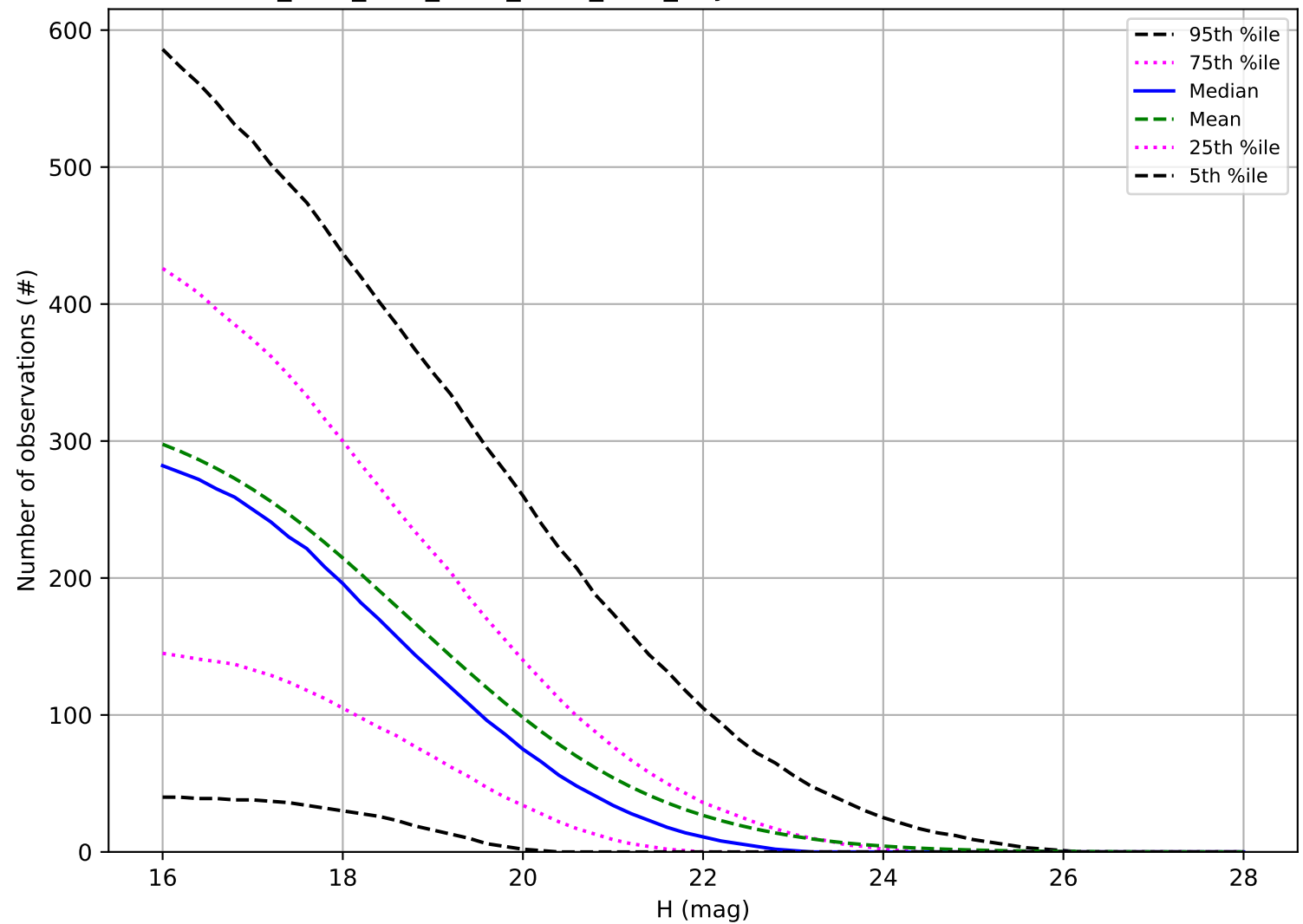
ddf_acor_sf30_lsf40_lsr50_v3.4_10yrs: Number of observations PHA
