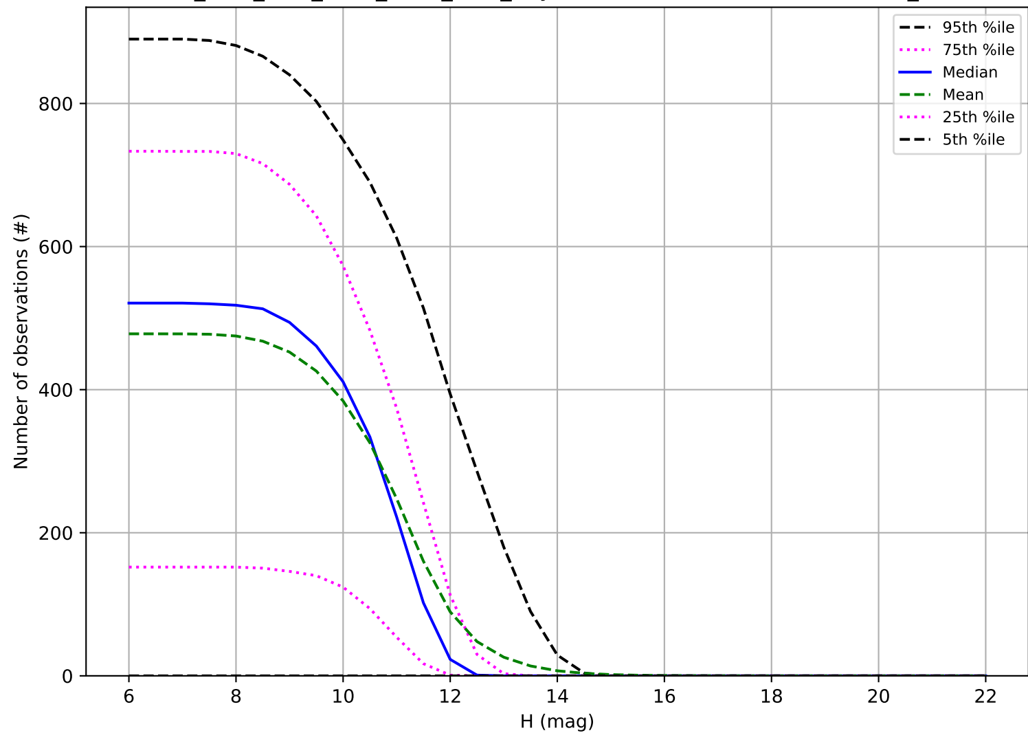
ddf_acor_sf30_lsf40_lsr50_v3.4_10yrs: Number of observations OCC_r20
