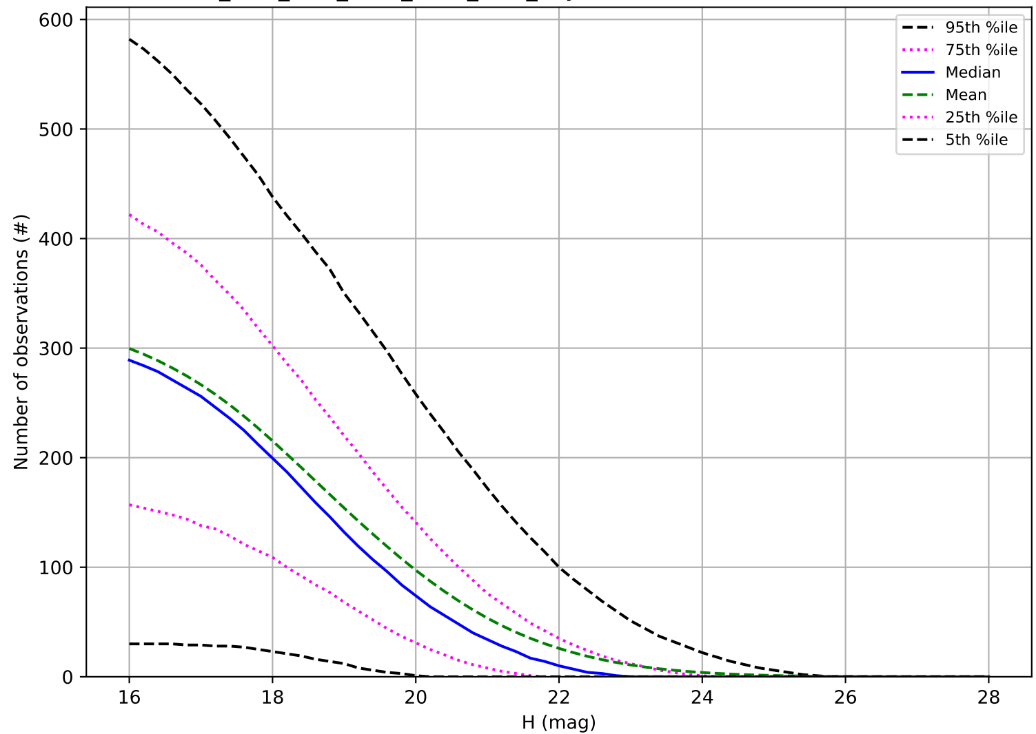
ddf_acor_sf30_lsf40_lsr50_v3.4_10yrs: Number of observations NEO
