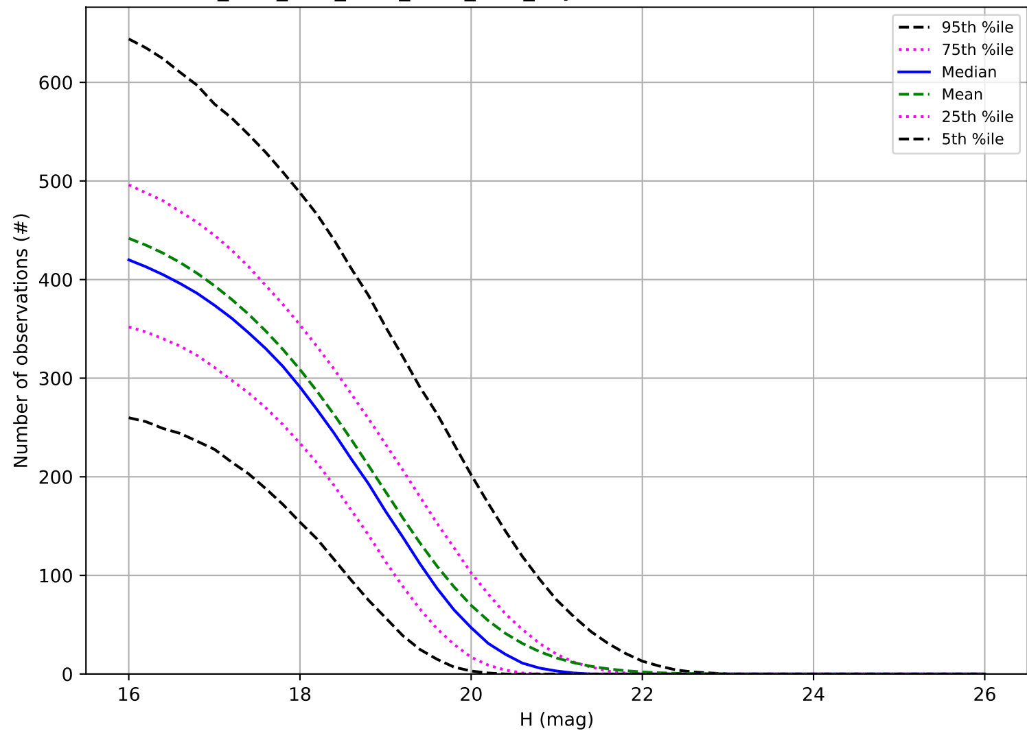
ddf_acor_sf30_Isf40_Isr50_v3.4_10yrs: Number of observations MBA
