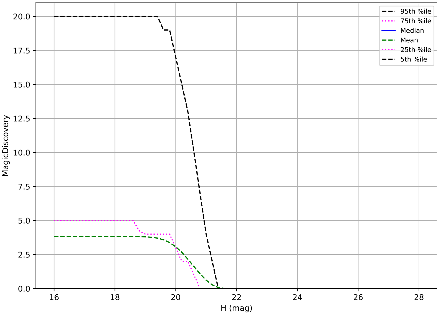
ddf_acor_sf30_lsf40_lsr50_v3.4_10yrs: Vatira 6 detections in 60 nights detection loss
