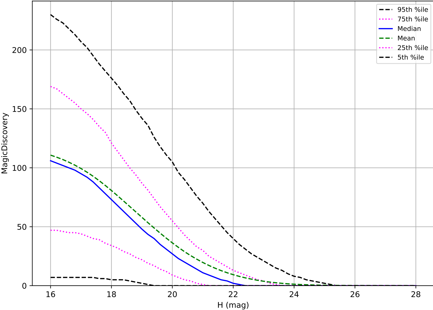
ddf_acor_sf30_lsf40_lsr50_v3.4_10yrs: PHA 6 detections in 60 nights detection loss
