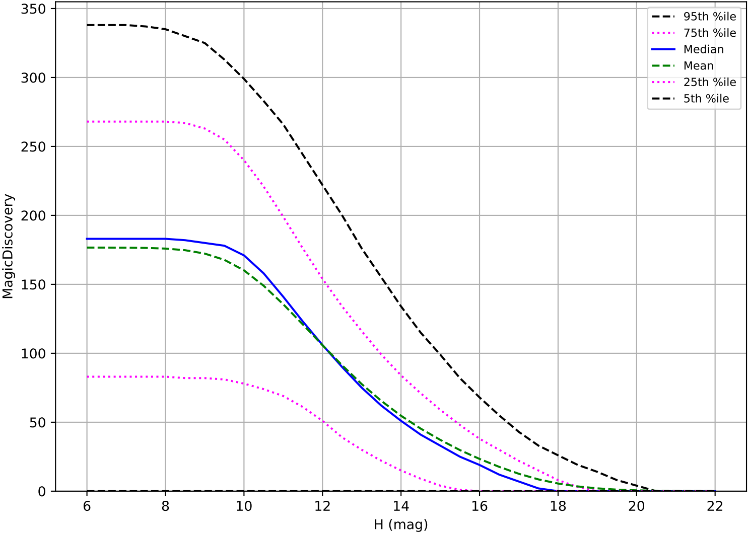
ddf_acor_sf30_lsf40_lsr50_v3.4_10yrs: OCC_r5 6 detections in 60 nights detection loss
