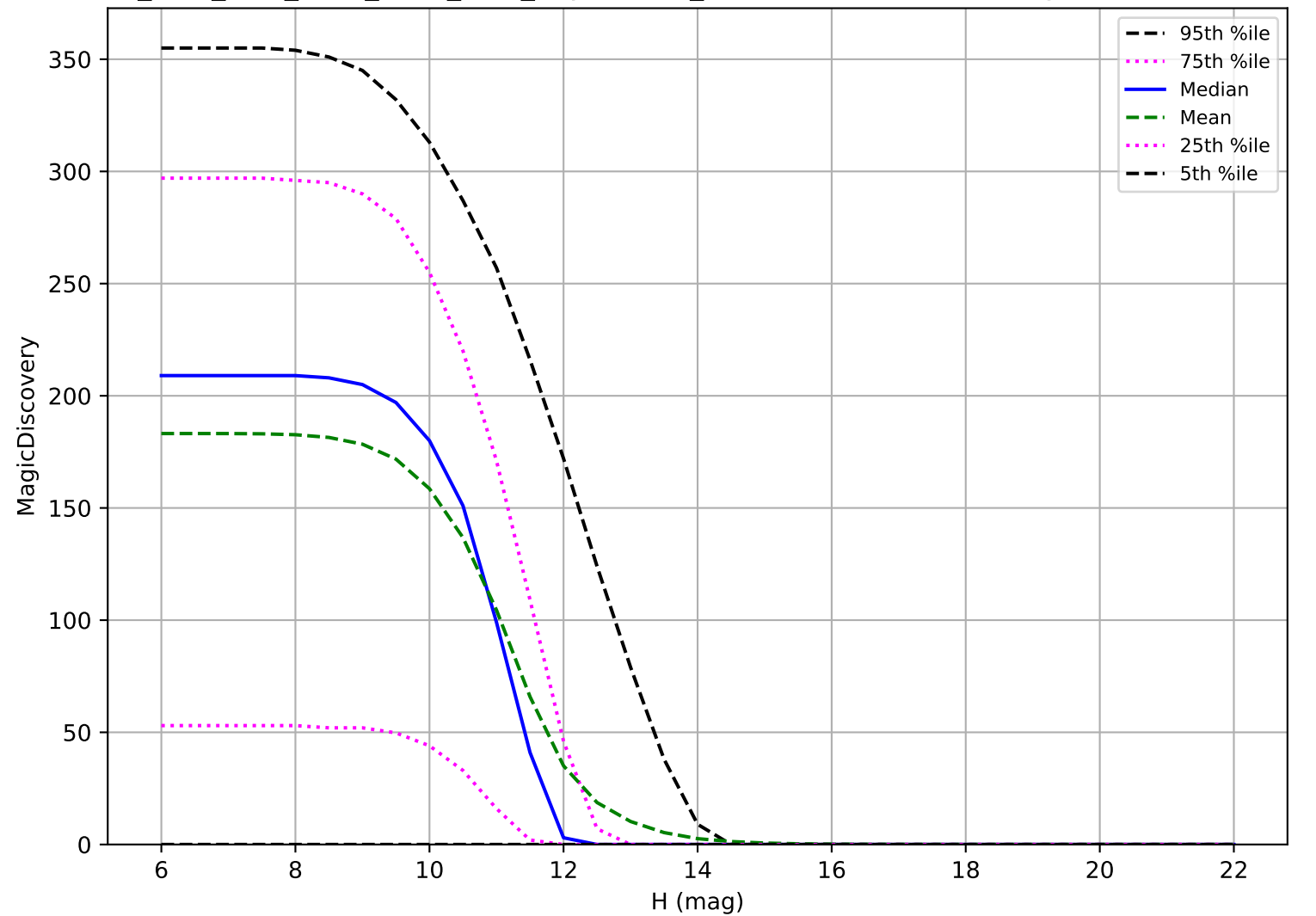
ddf_acor_sf30_lsf40_lsr50_v3.4_10yrs: OCC_r20 6 detections in 60 nights detection loss
