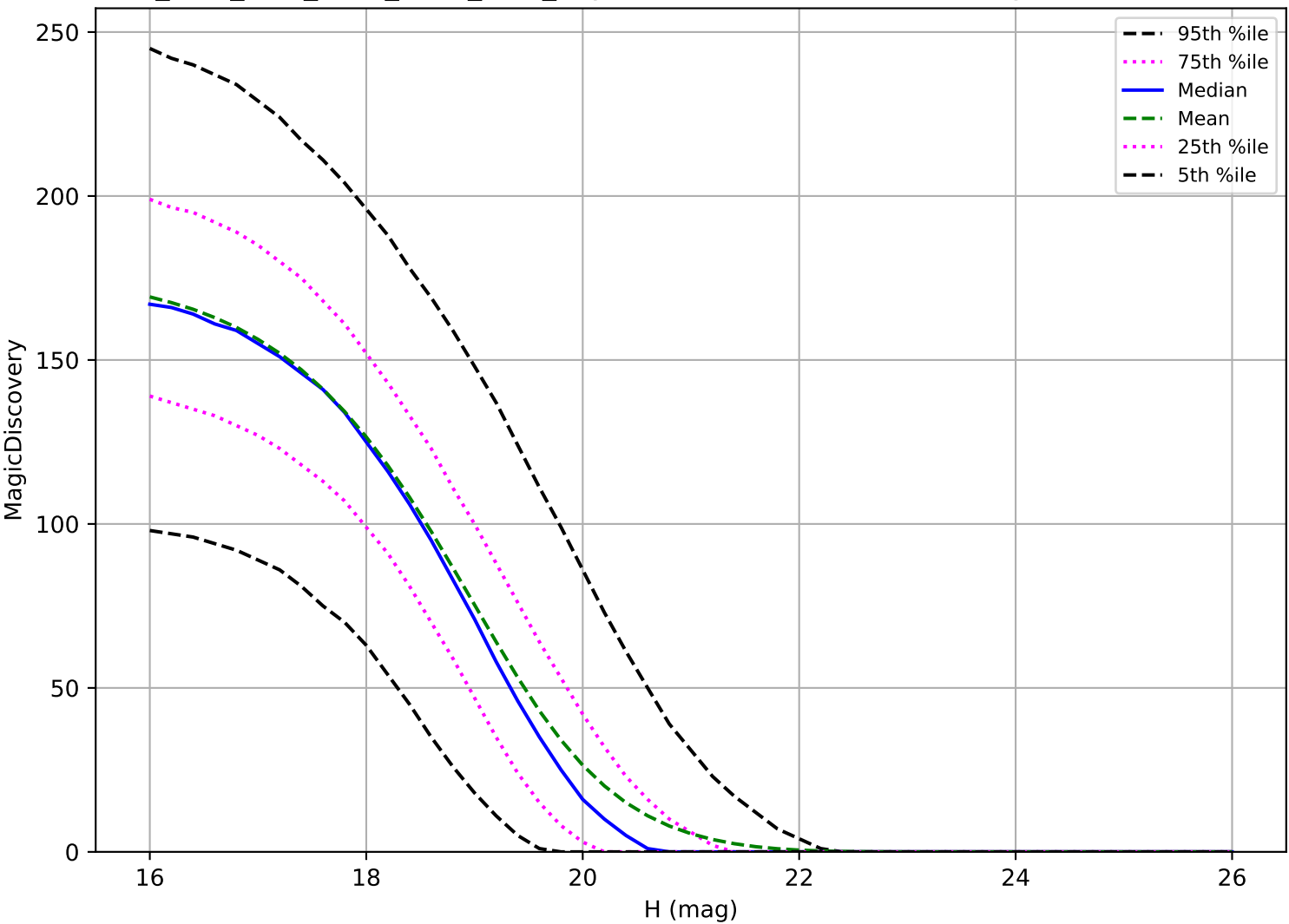
ddf_acor_sf30_lsf40_lsr50_v3.4_10yrs: MBA 6 detections in 60 nights detection loss
