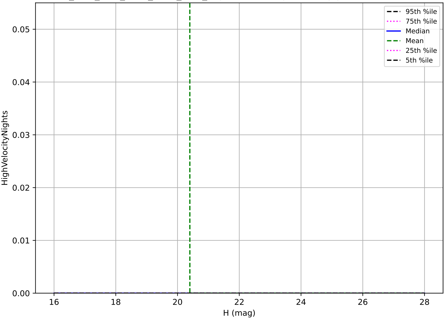
ddf_acor_sf30_lsf40_lsr50_v3.4_10yrs: Vatira High velocity pair detection loss
