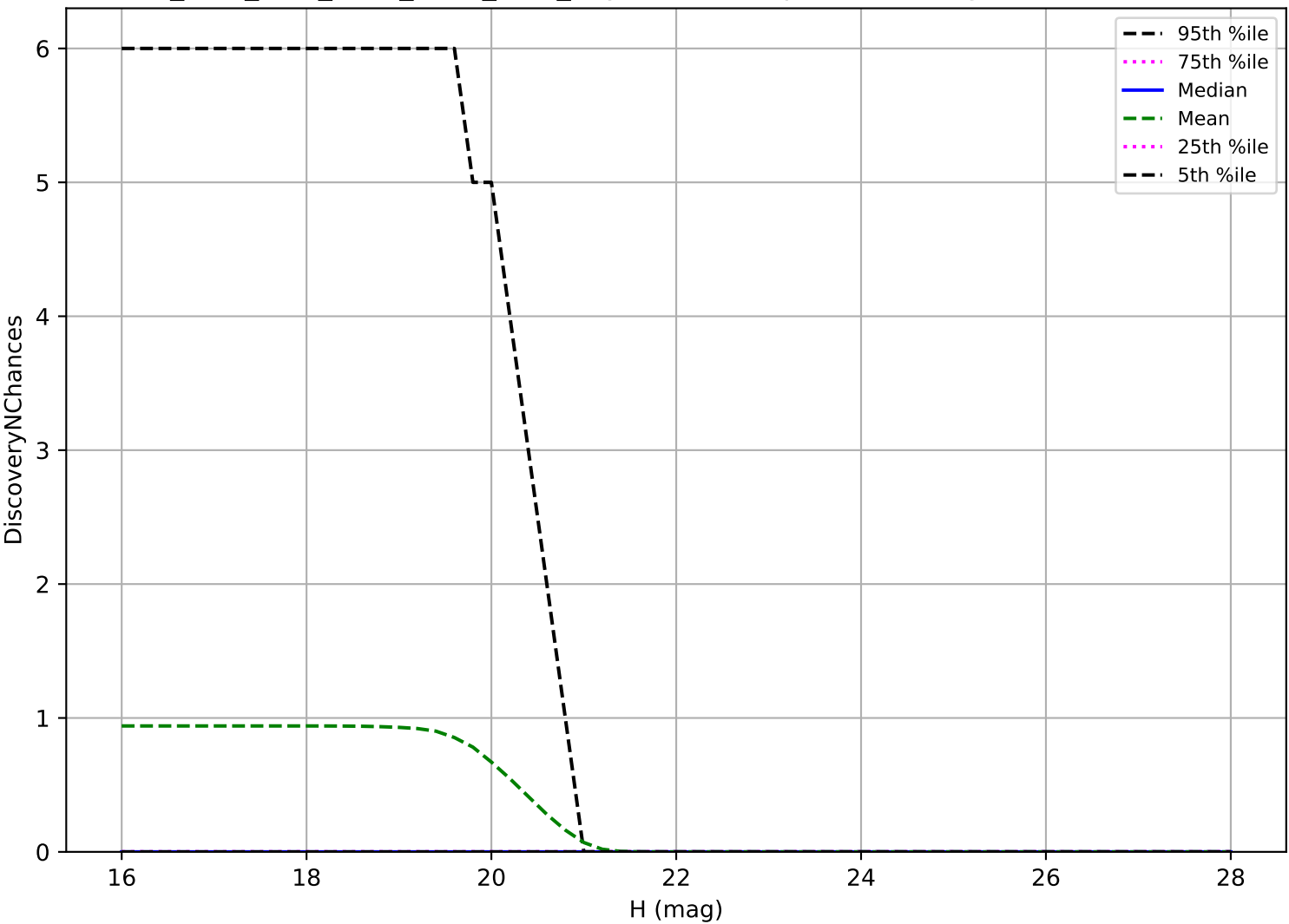
ddf_acor_sf30_lsf40_lsr50_v3.4_10yrs: Vatira 3 pairs in 15 nights detection loss
