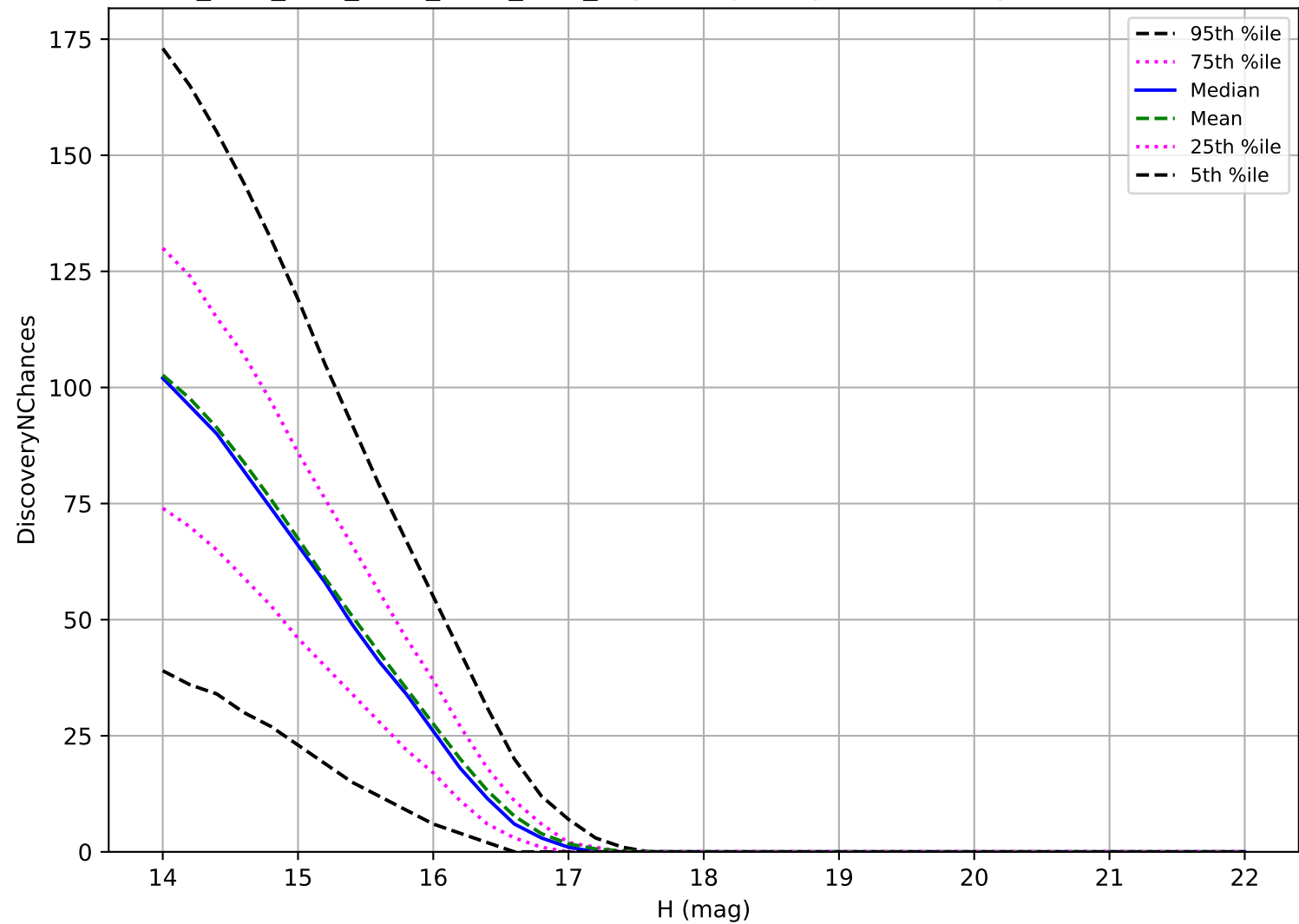
ddf_acor_sf30_lsf40_lsr50_v3.4_10yrs: Trojan 3 pairs in 15 nights detection loss
