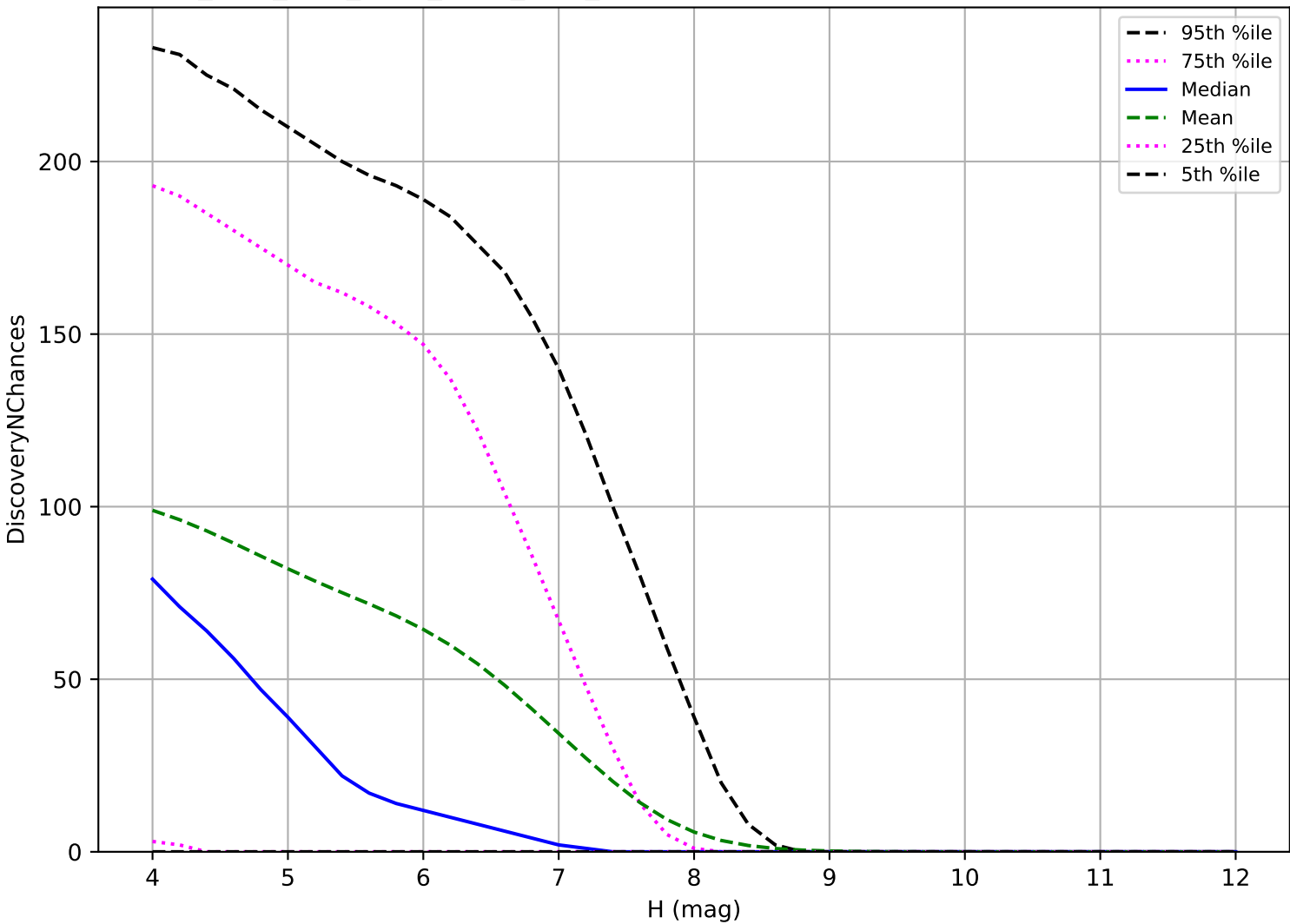
ddf_acor_sf30_lsf40_lsr50_v3.4_10yrs: TNO 3 pairs in 15 nights detection loss
