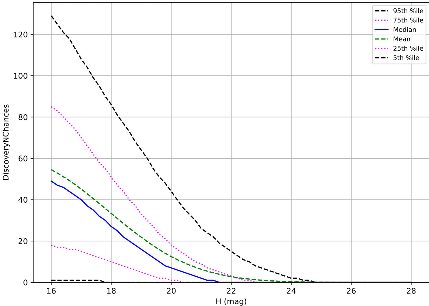
ddf_acor_sf30_lsf40_lsr50_v3.4_10yrs: PHA 3 pairs in 15 nights detection loss
