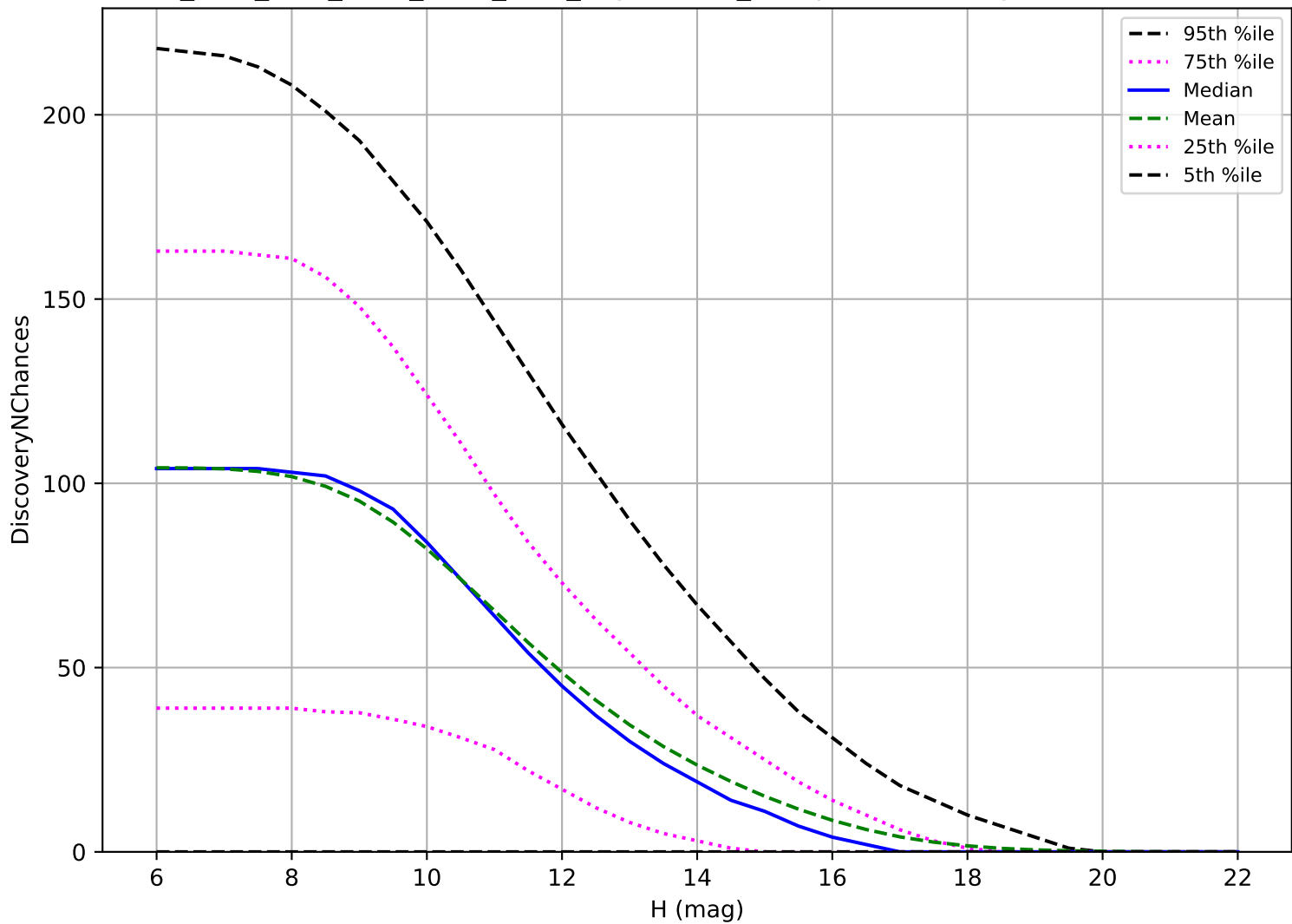
ddf_acor_sf30_lsf40_lsr50_v3.4_10yrs: OCC_r5 3 pairs in 15 nights detection loss
