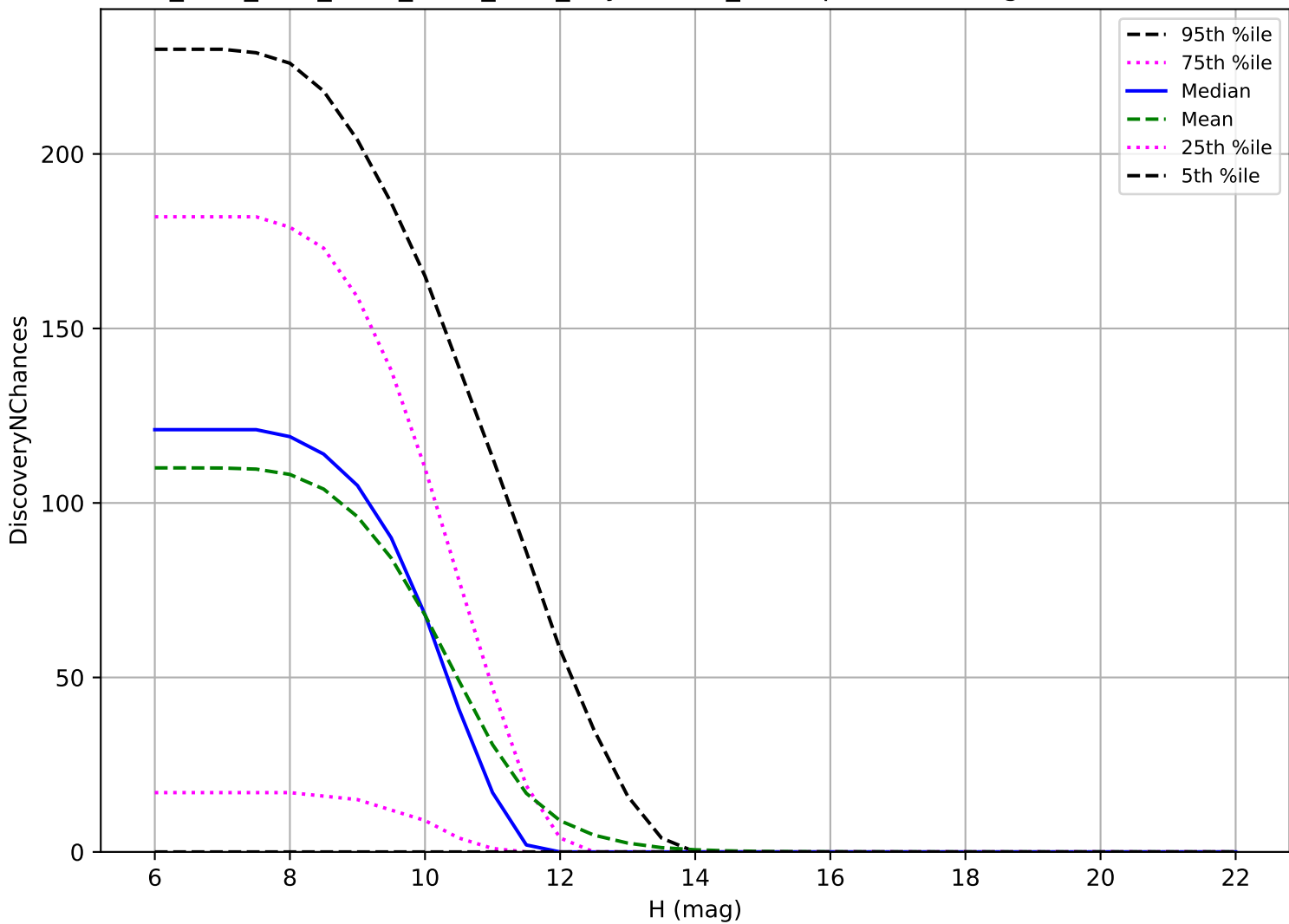
ddf_acor_sf30_lsf40_lsr50_v3.4_10yrs: OCC_r20 3 pairs in 15 nights detection loss
