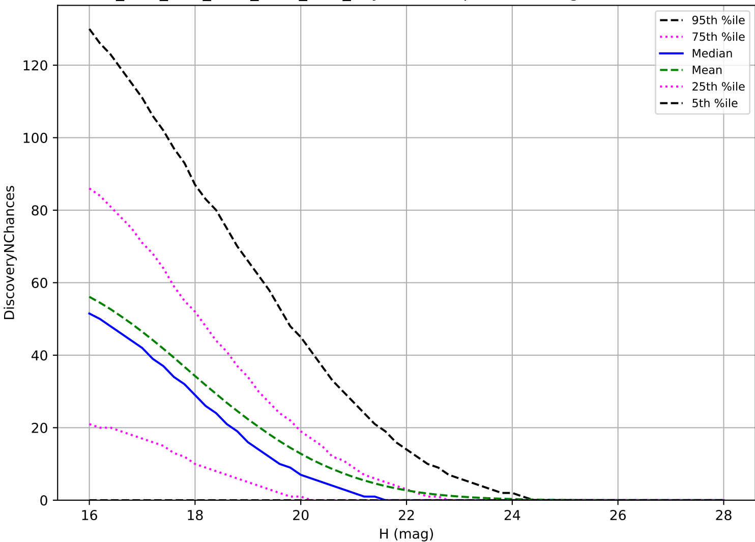
ddf_acor_sf30_lsf40_lsr50_v3.4_10yrs: NEO 3 pairs in 15 nights detection loss
