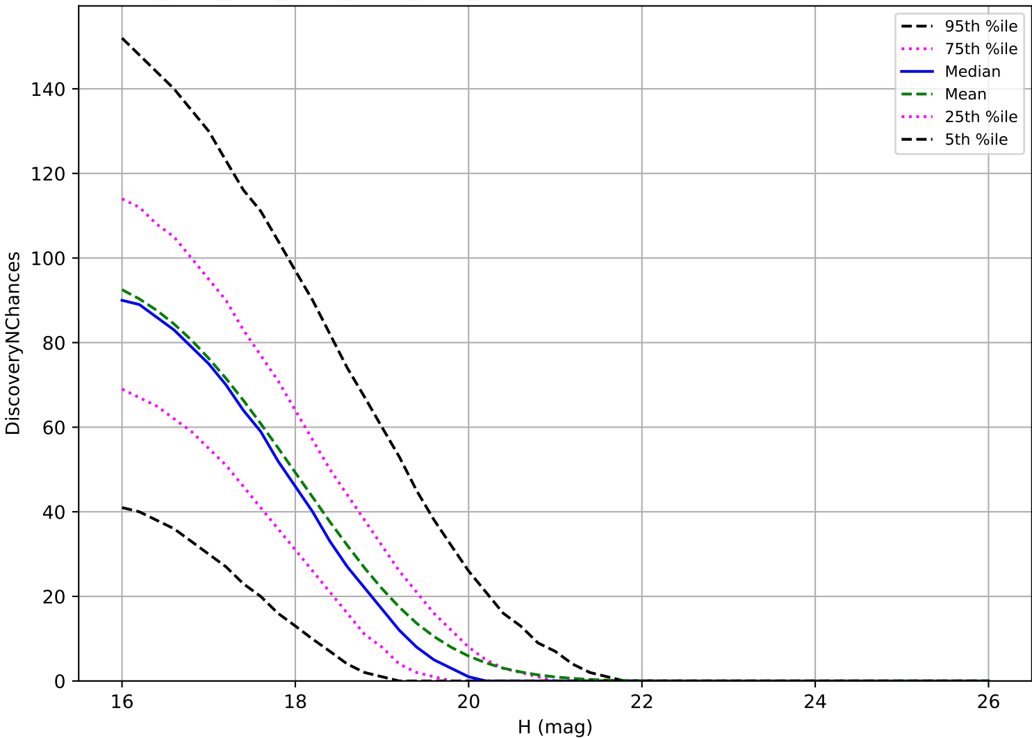
ddf_acor_sf30_lsf40_lsr50_v3.4_10yrs: MBA 3 pairs in 15 nights detection loss
