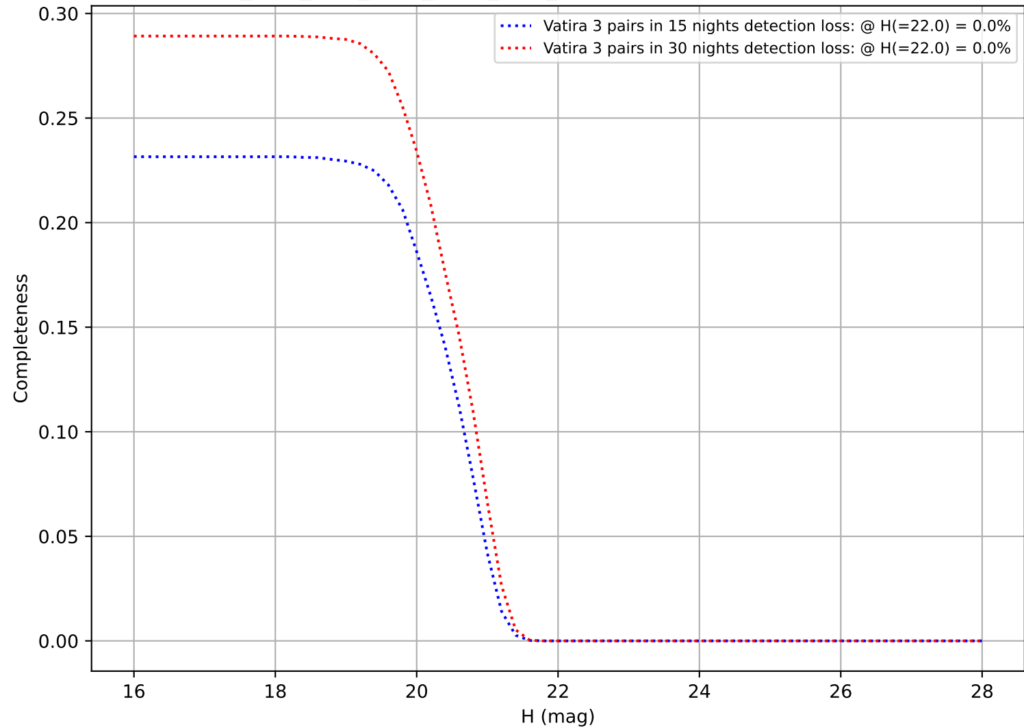
ddf_acor_sf30_lsf40_lsr50_v3.4_10yrs: DifferentialCompleteness
