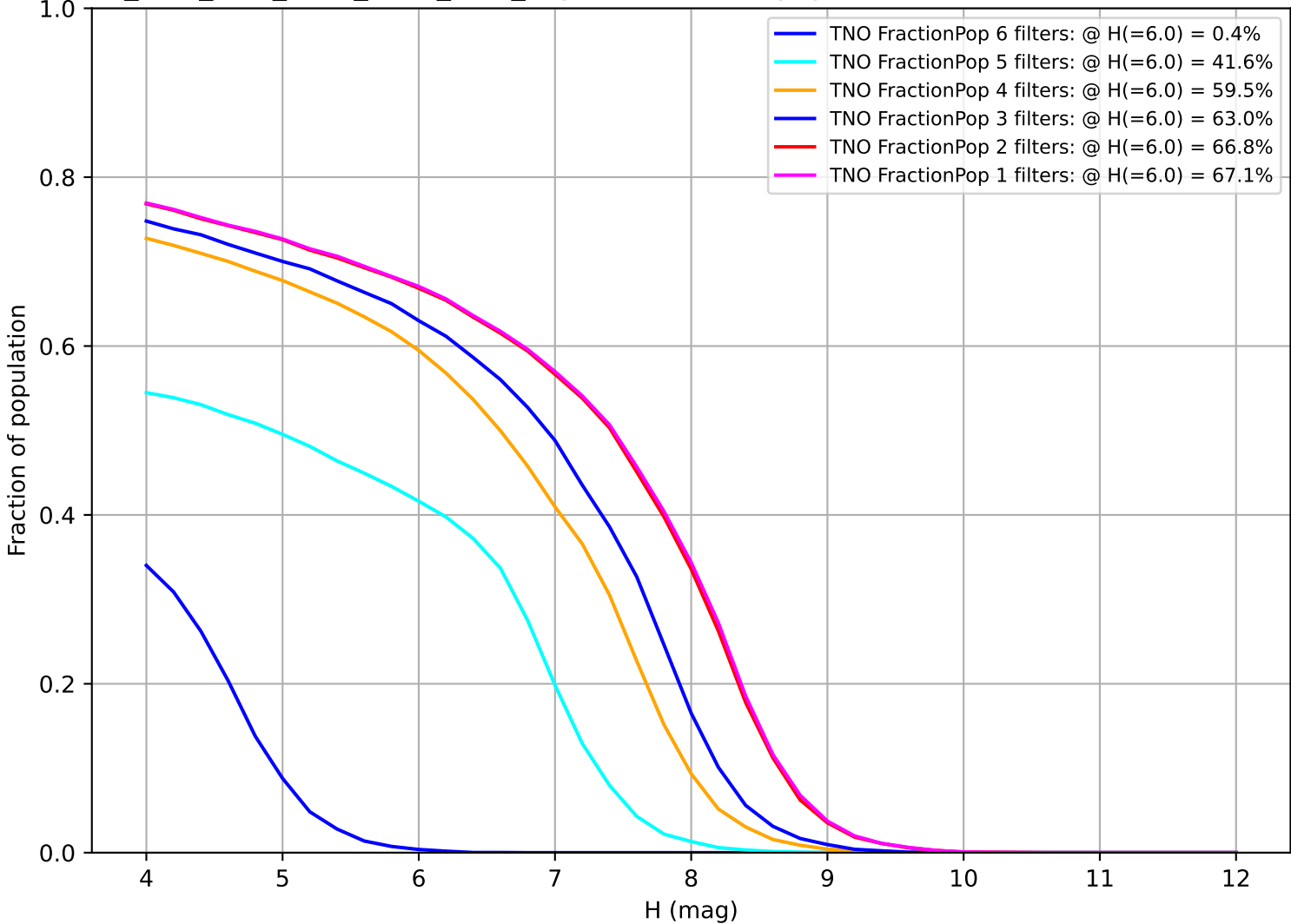
ddf_acor_sf30_lsf40_lsr50_v3.4_10yrs: Fraction of population with colors in X filters TNO
