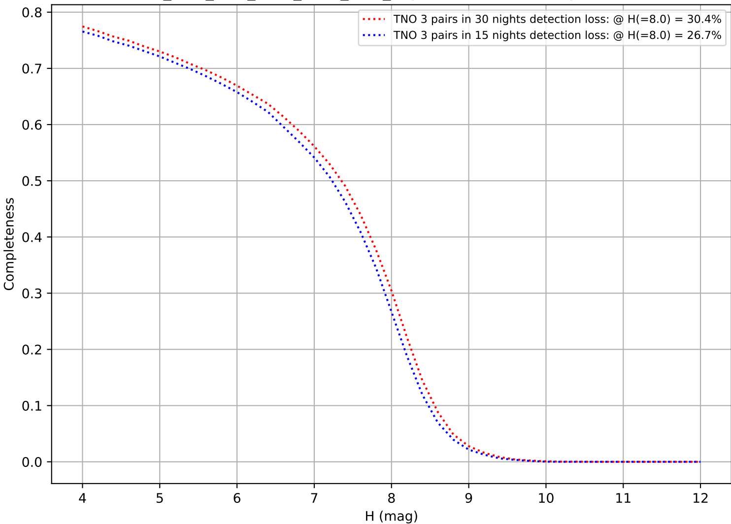
ddf_acor_sf30_lsf40_lsr50_v3.4_10yrs: DifferentialCompleteness
