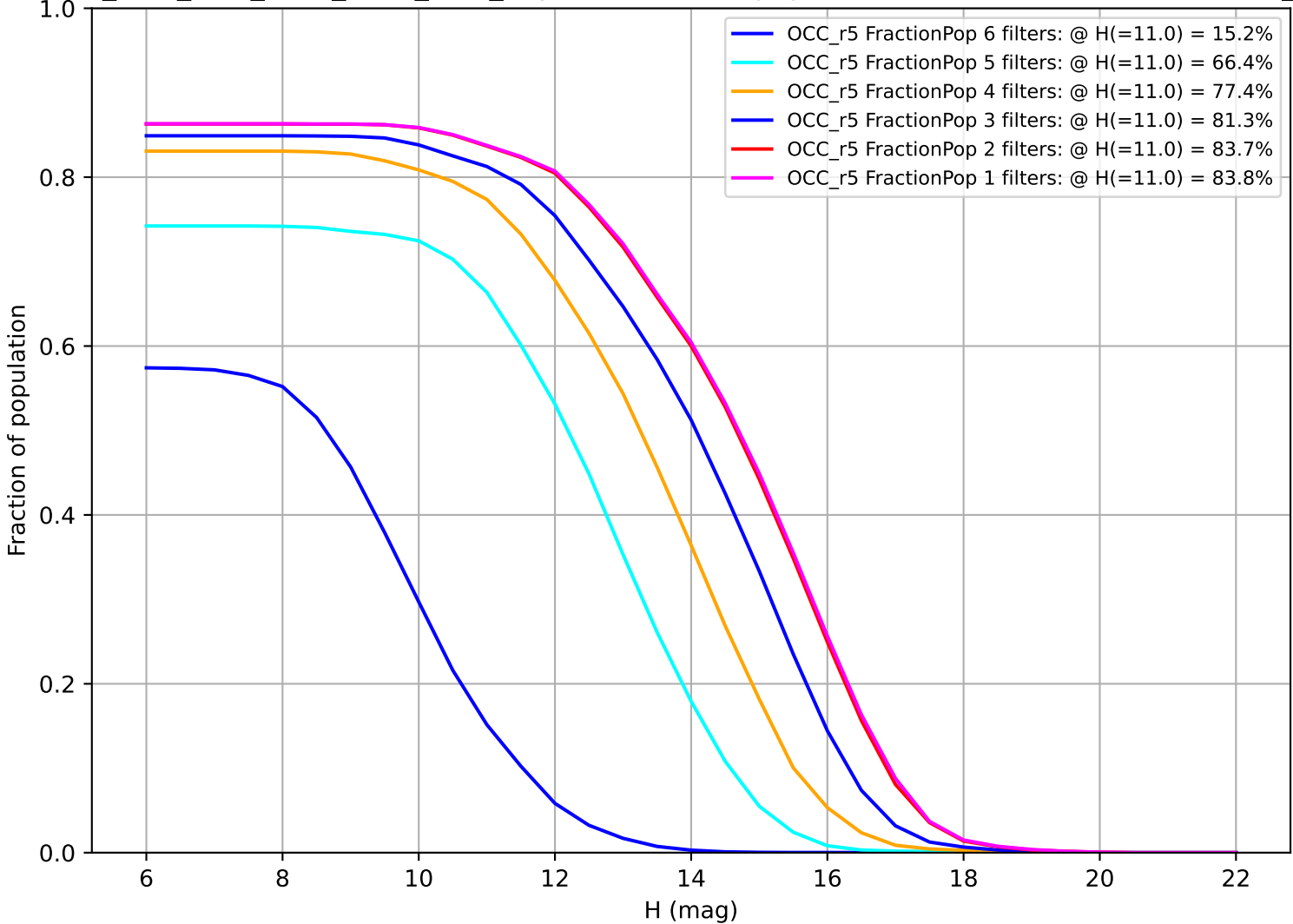
ddf_acor_sf30_lsf40_lsr50_v3.4_10yrs: Fraction of population with colors in X filters OCC_r5
